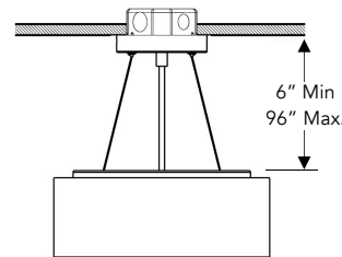
Cable Mount
